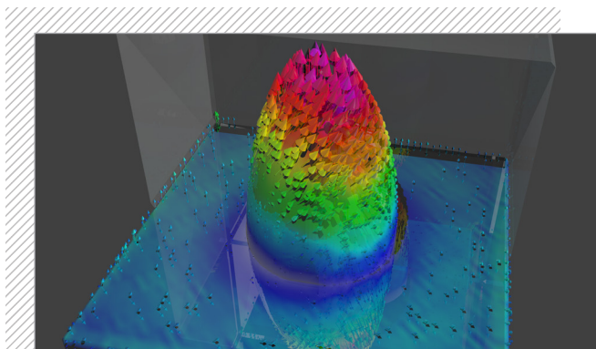
Figure 3. InAs-GaAs quantum dot strain displacement.
